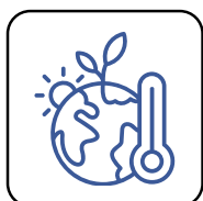
Climat
