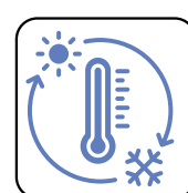
Climat
